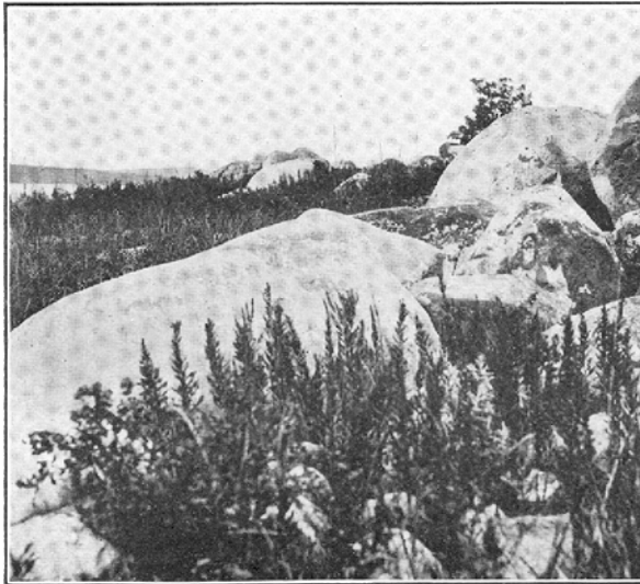
Fig. 2. Abandoned sea wall on "Rocky Island" looking east. Near view of wall. (Henderson).
