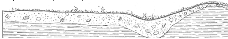
Fig. 3. Diagram showing the relation of drift to bedrock in a glaciated region.
