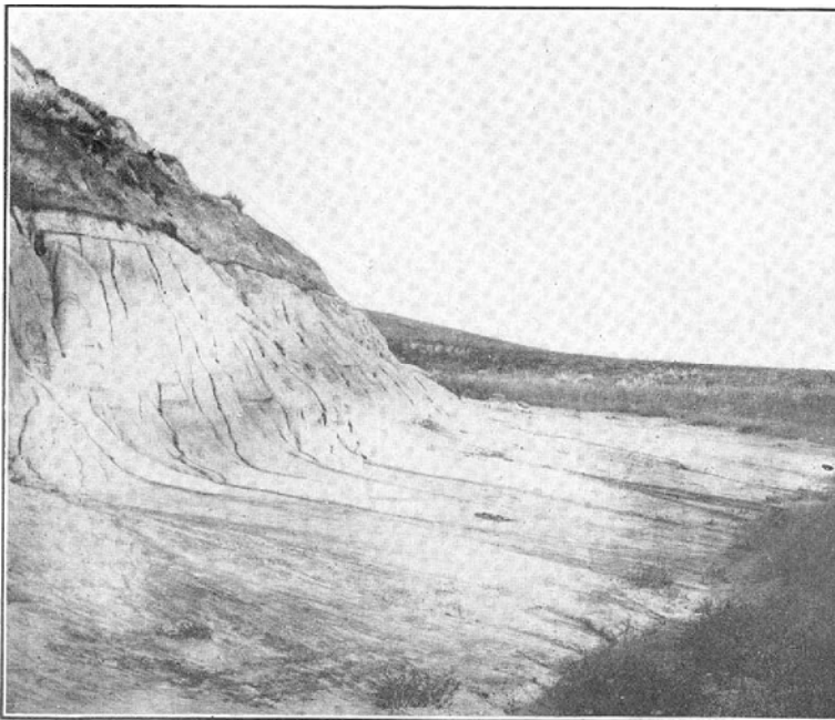
Fig. 2. Outwash material at the base of one of the Twin Buttes, 8 miles south of Bismarck, showing the result of rain erosion.
