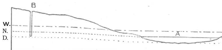
1.—Diagram showing the relation of lakes and wells to the
