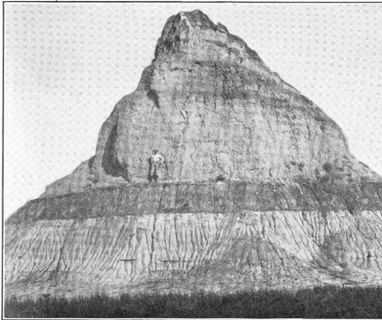
Fig. 1. One of the Twin Buttes, 8 miles south of Bismarck, on the east side of Missouri River. The butte is formed of Lance beds and shows well the effect of rain erosion on the soft clays and sands.
