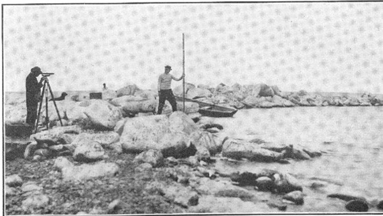
Fig. 2. Eastern shore of Rock Pile Island, looking north.
