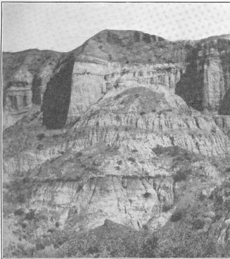
Bluff on the west side of the Missouri River formed of Lance beds, four miles north of Gwyther, Morton County. NORTH DAKOTA GEOLOGICAL SURVEY PLATE 1.
