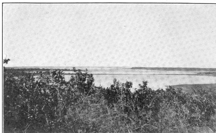
Fig. 2. Court Lake, a freshwater lake, showing final stage of separation. timbered beach in background is same as that in foreground of Fig. 1.(Knudson)
