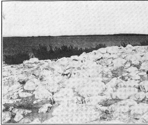
Fig. 1. Boulder pavement on north shore of Bird Island, Devils Lake. Old cormorants net among alkali incrustec. boulders. (Henderson).
