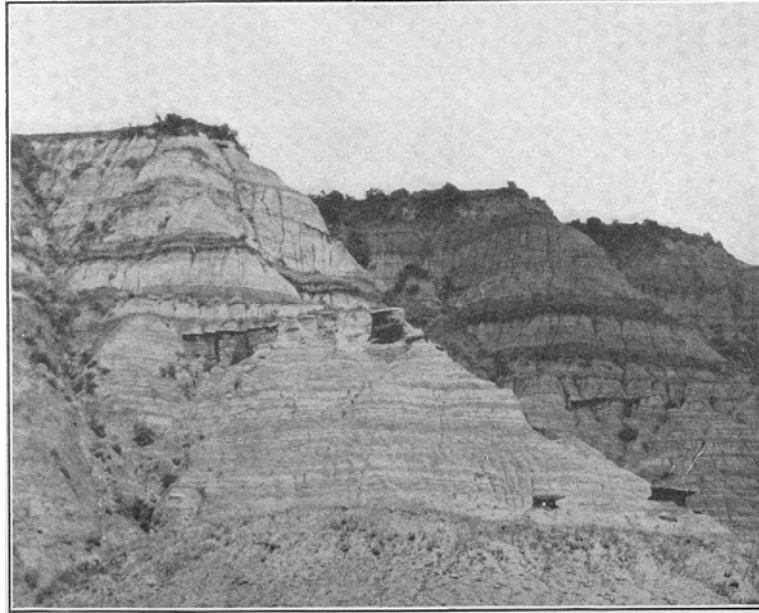
Fig. 1. Contact of Fox Hills sandstone and Lance formation, on Cannon Ball River. The ledge on which the man stands forms the top of the Fox Hills.
