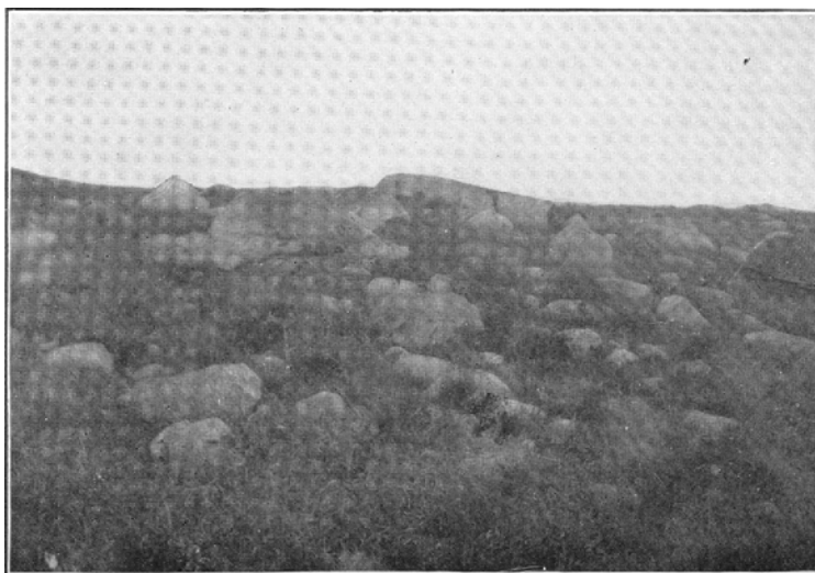
Fig. 2. Boulder covered hill of the moraine in Little Heart basin, Morton County.
