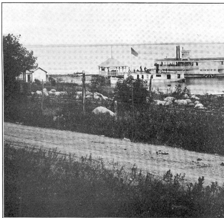
Devils Lake looking southwest from Chautauqua NORTH DAKOTA GEOLOGICAL SURVEY PLATE XTIL Devils Lake looking southwest from Chautauqua (Photo by Kitchen, 1903.)
