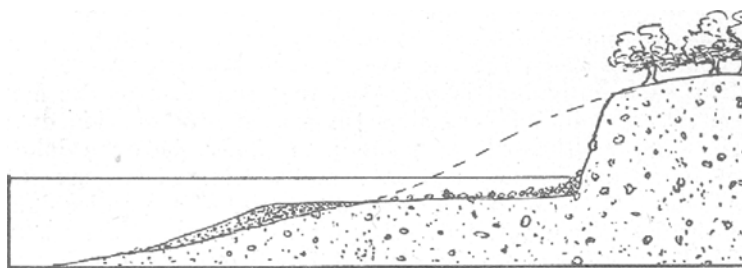
Fig. 6. Cross section of cliff and wave cut terrace.
