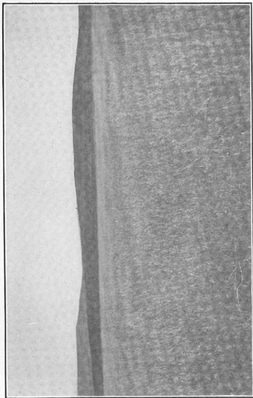
Fig. 1. Moraine hill rising above the flat valley train of the Southeast Branch
