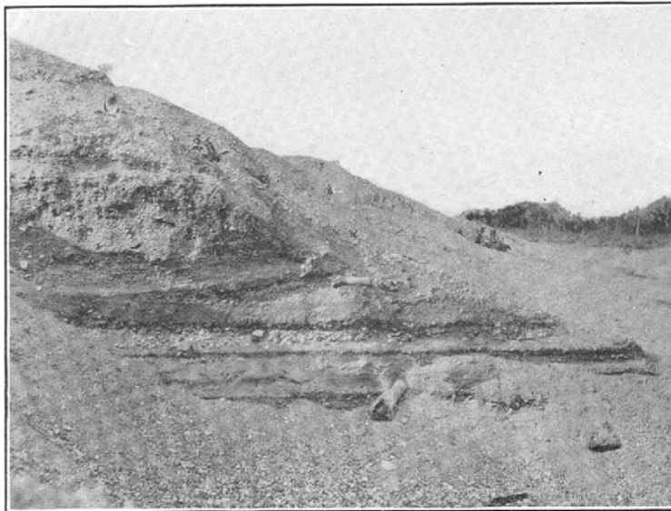
Fig. 1. Section of beach, C 1884, in gravel pit east side Creel PLATE XXI.
