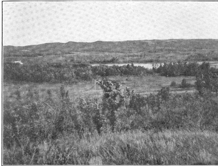
1. :morainic topography south of Mission Day, Devils Lake. Residual ridge veneered with recessional moraine in background, deep irregular basin in foreground. Indian house on left. (Knudson.)
