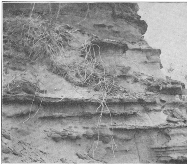
Pox Hills sandstone in the bluffs of the Cannon Ball River, showing how weathering has left the harder portion projecting.
