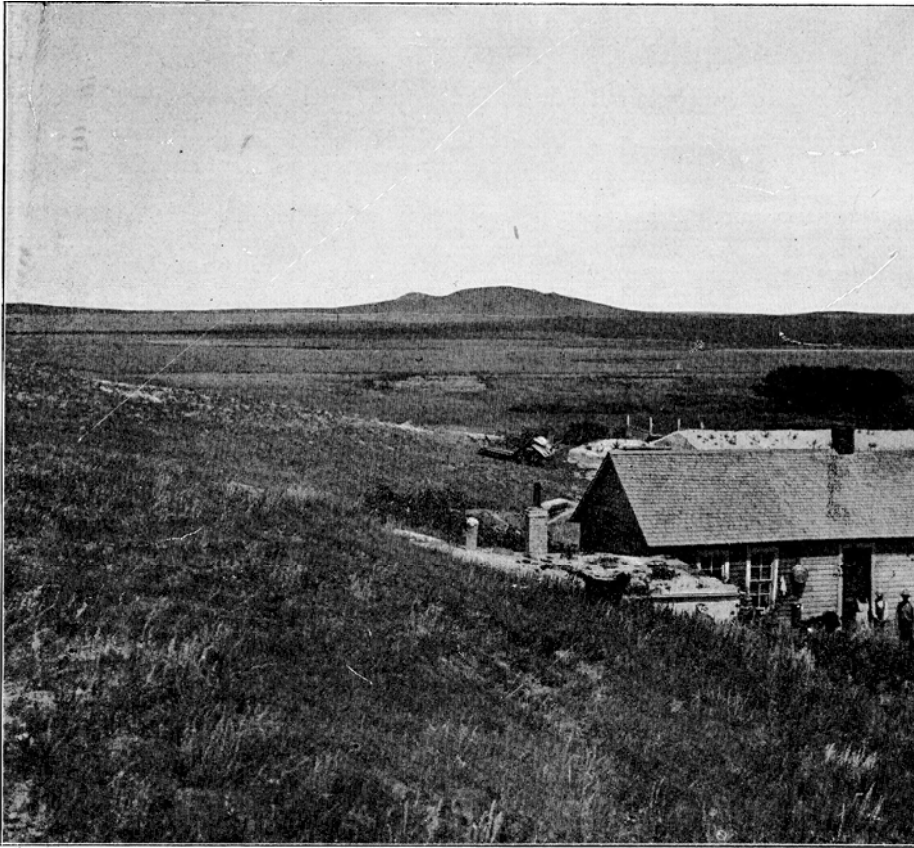
The Valley of Green River, Illustrating a Common Type of Topography in the Lignite Area, and a Valley of a Small Stream, Capable of Irrigation.
