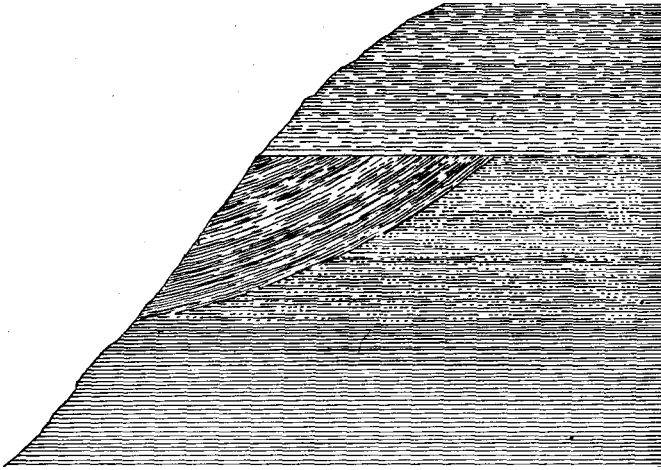
Fig. 1. Peculiar bedding in Laramie clays.
